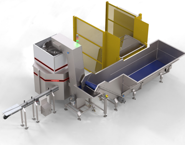
PFI Container Unscrambler with hydraulic driven dumper
